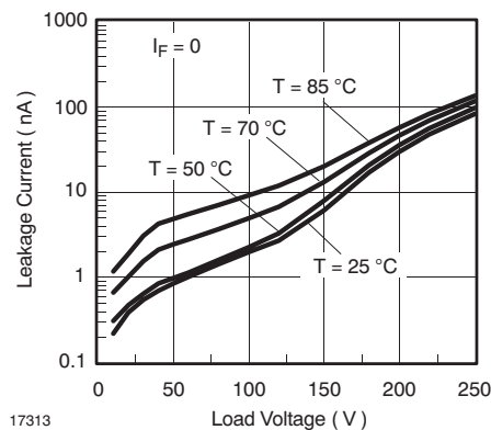
Figure 14. Leakage Current vs. Applied Voltage
