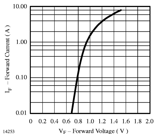
Figure 14. I_F vs. V_F
