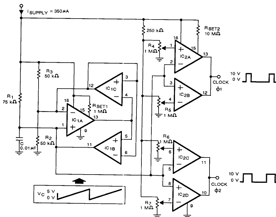
Square Wave Oscillator
