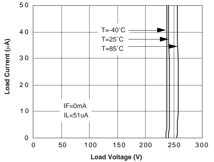
Figure 18. Switch Breakdown Voltage vs. Temperature
