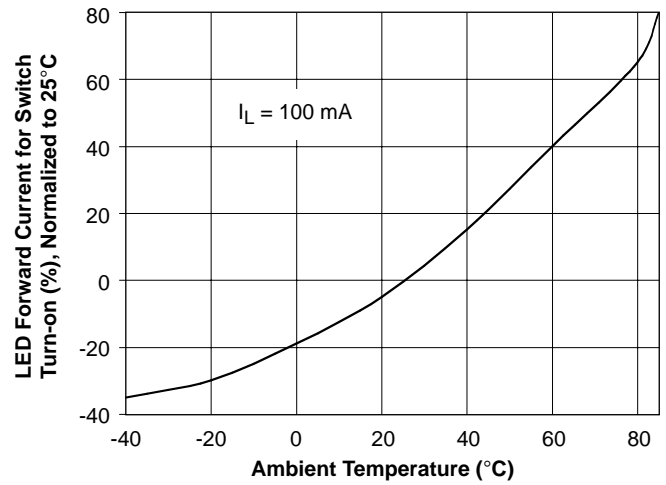
Figure 5. LED Current for Switch Turn-on vs. Temperature
