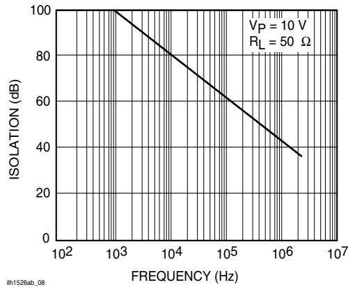
Figure 9. Output Isolation
