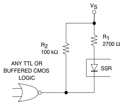
Figure 19. Input Control Circuit
