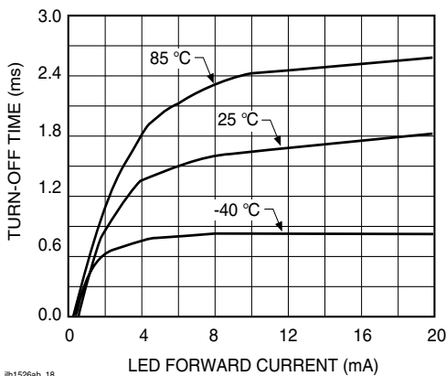
Figure 18. Turn-off Time vs. LED Current
