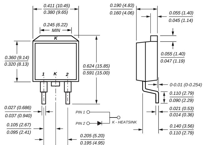
TO-263AB (MBRB10xx)
