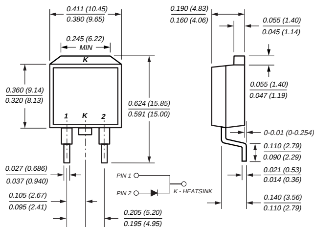
TO-263AB (MBRB10Hxx)
