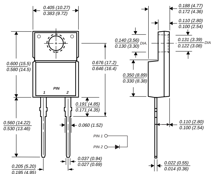
ITO-220AC (MBRF10Hxx)
