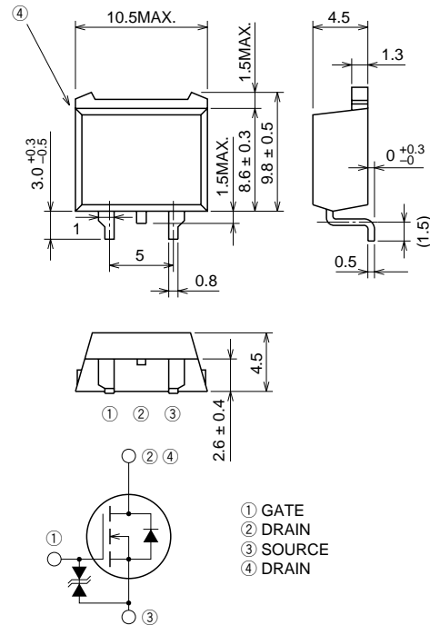
TO-220S
