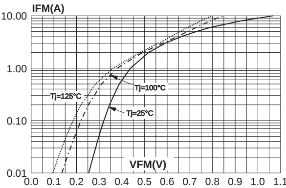
Fig. 7-2: Forward voltage drop versus forward current (typical values) (1N5819).
