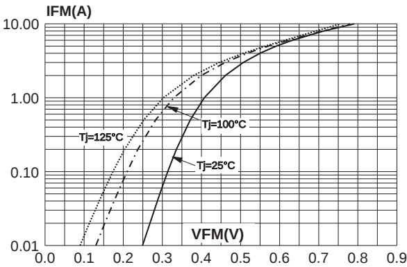
Fig. 7-1: Forward voltage drop versus forward current (typical values) (1N5817/1N5818).
