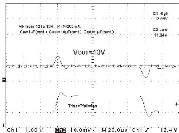
Line Transient
