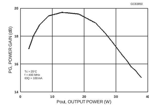
Power Gain vs Output Power
