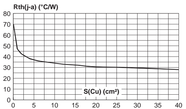
Fig. 8: Thermal resistance junction to ambient versus copper surface under tab (Epoxy printed circuit board FR4, copper thickness: 35µm) (STPS40L45CG only).
