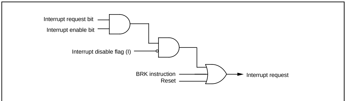
Fig. 6 Interrupt control
