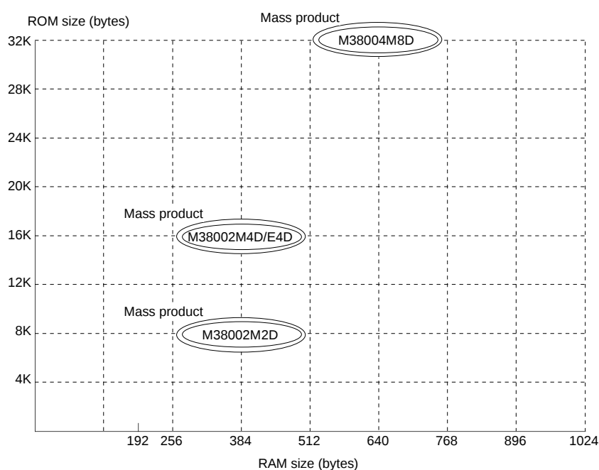
Fig. 6 Memory expansion plan (Extended operating temperature version)
