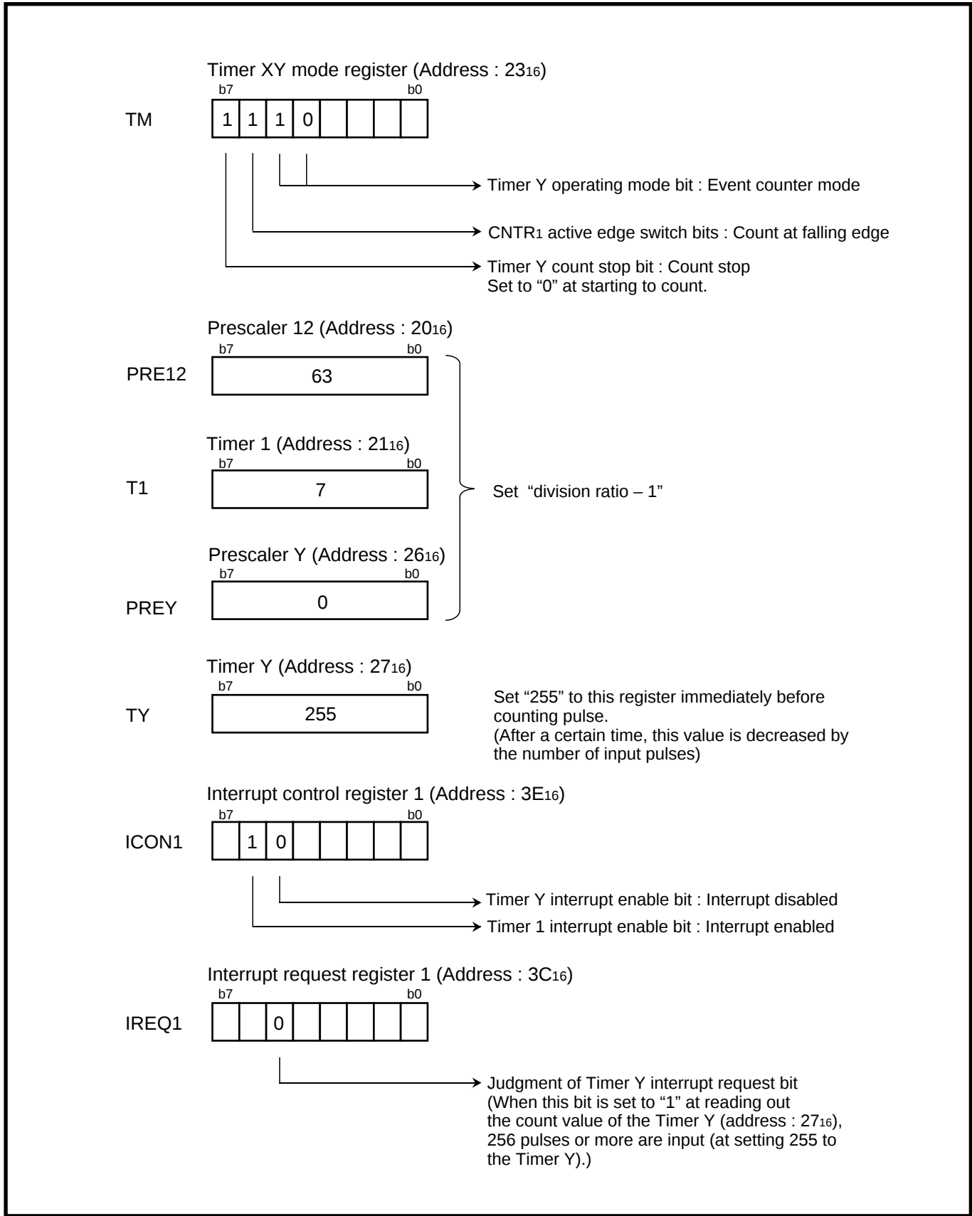
Fig. 2.2.18 Setting of related registers [Measurement of frequency]
