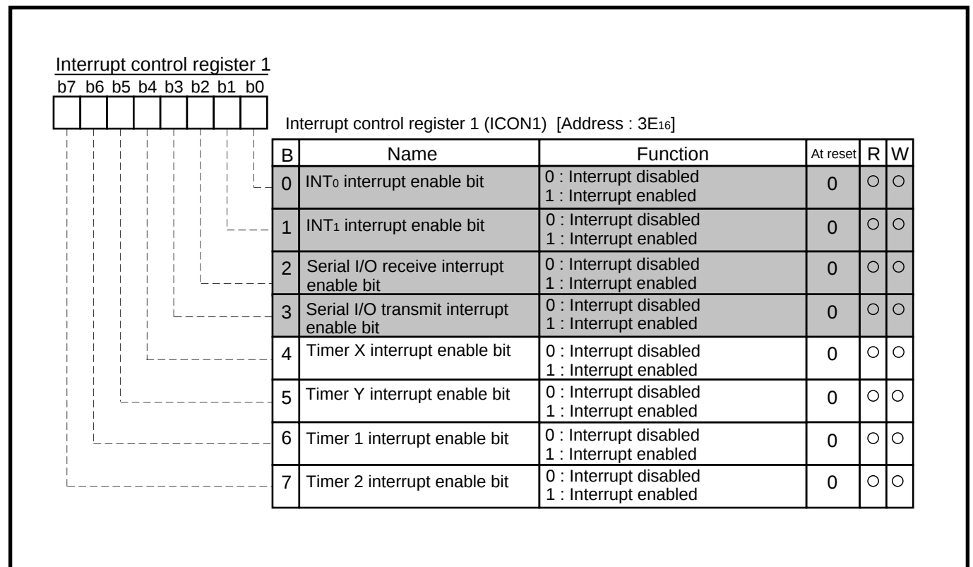
Fig. 2.2.8 Structure of Interrupt control register 1
