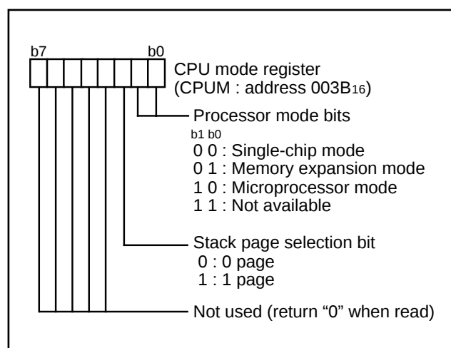
Fig. 29 Structure of CPU mode register
