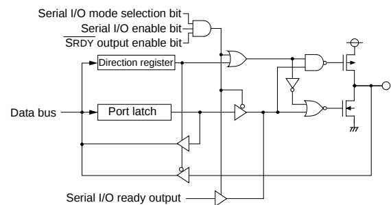
(6) Port P47
