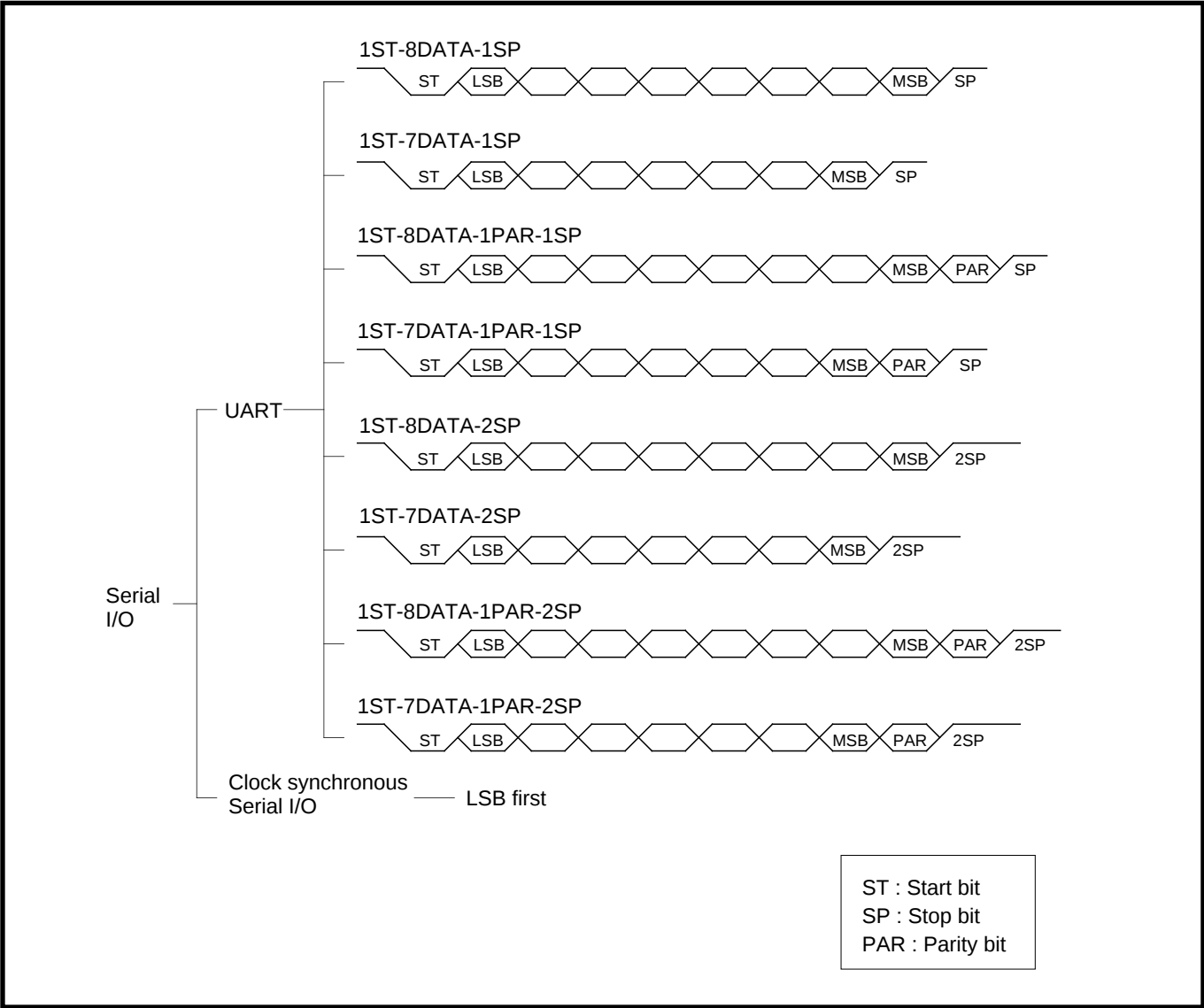
Fig. 2.3.12 Setting of Serial I/O transfer data format
