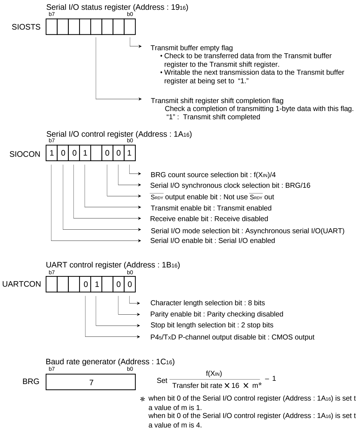
Fig. 2.3.31 Setting of related registers at a transmitting side [Communication using UART]
