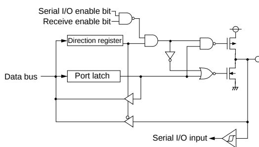
(3) Port P44
