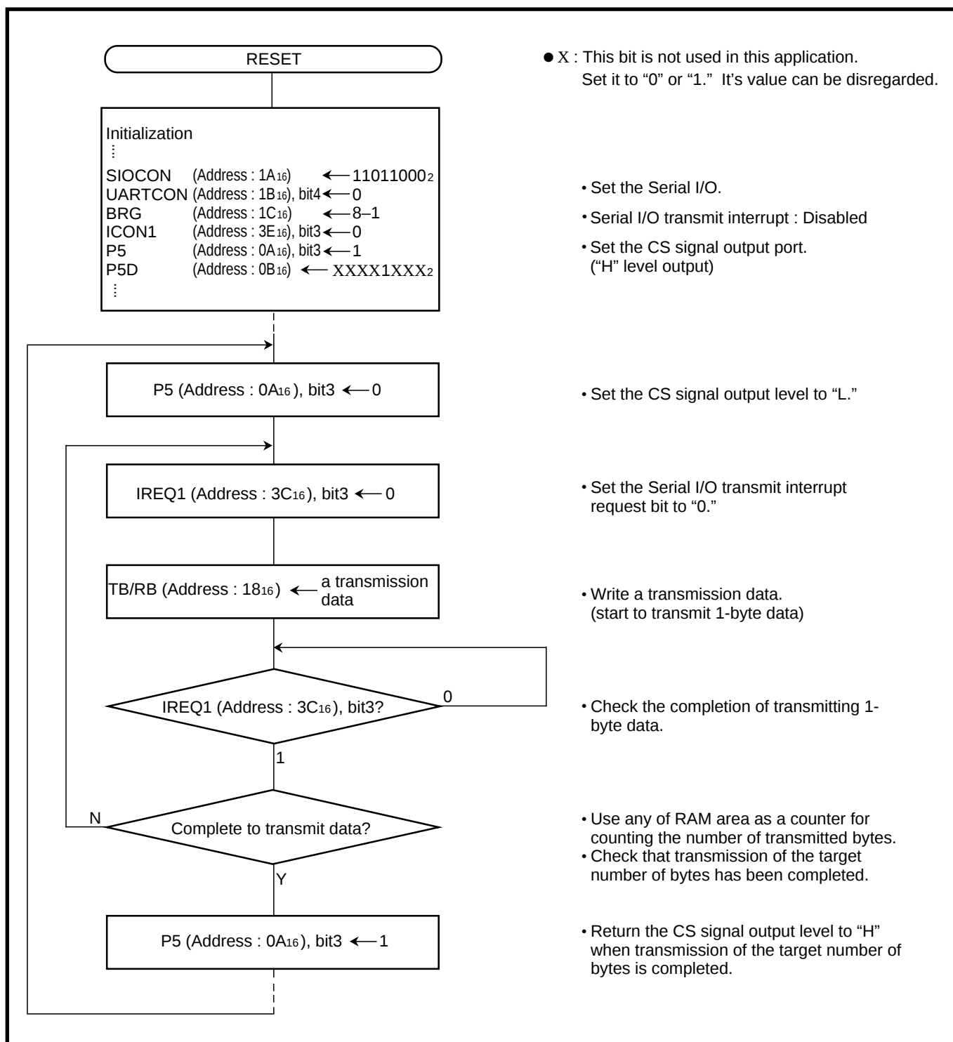
Fig. 2.3.23 Control procedure of serial I/O [Output of serial data]
