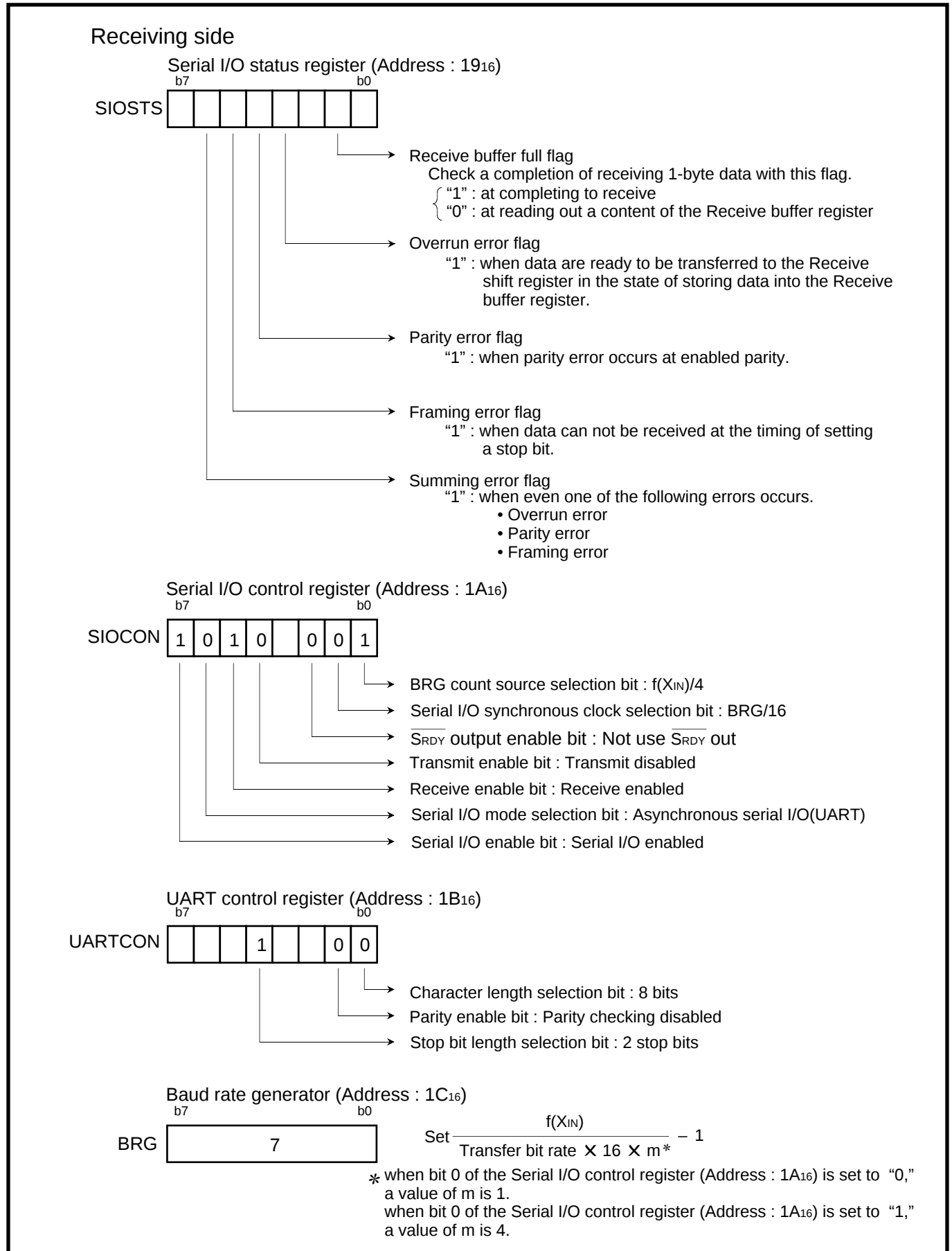
Fig. 2.3.32 Setting of related registers at a receiving side [Communication using UART]
