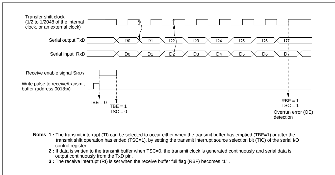
Fig. 18 Operation of clock synchronous serial I/O function
