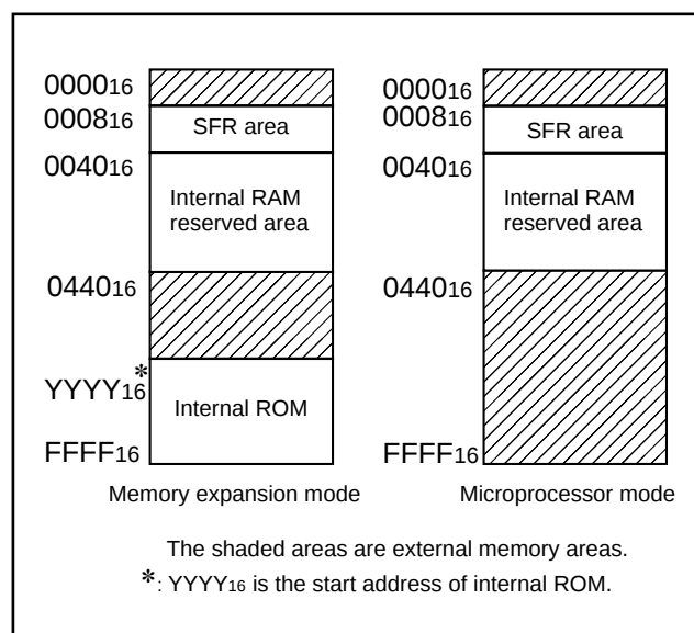
Fig. 28 Memory maps in various processor modes
