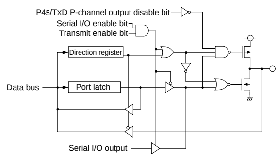
(4) Port P45
