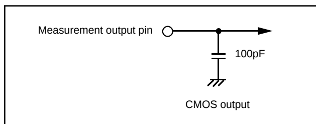
Fig. 3.1.1 Circuit for measuring output switching characteristics
