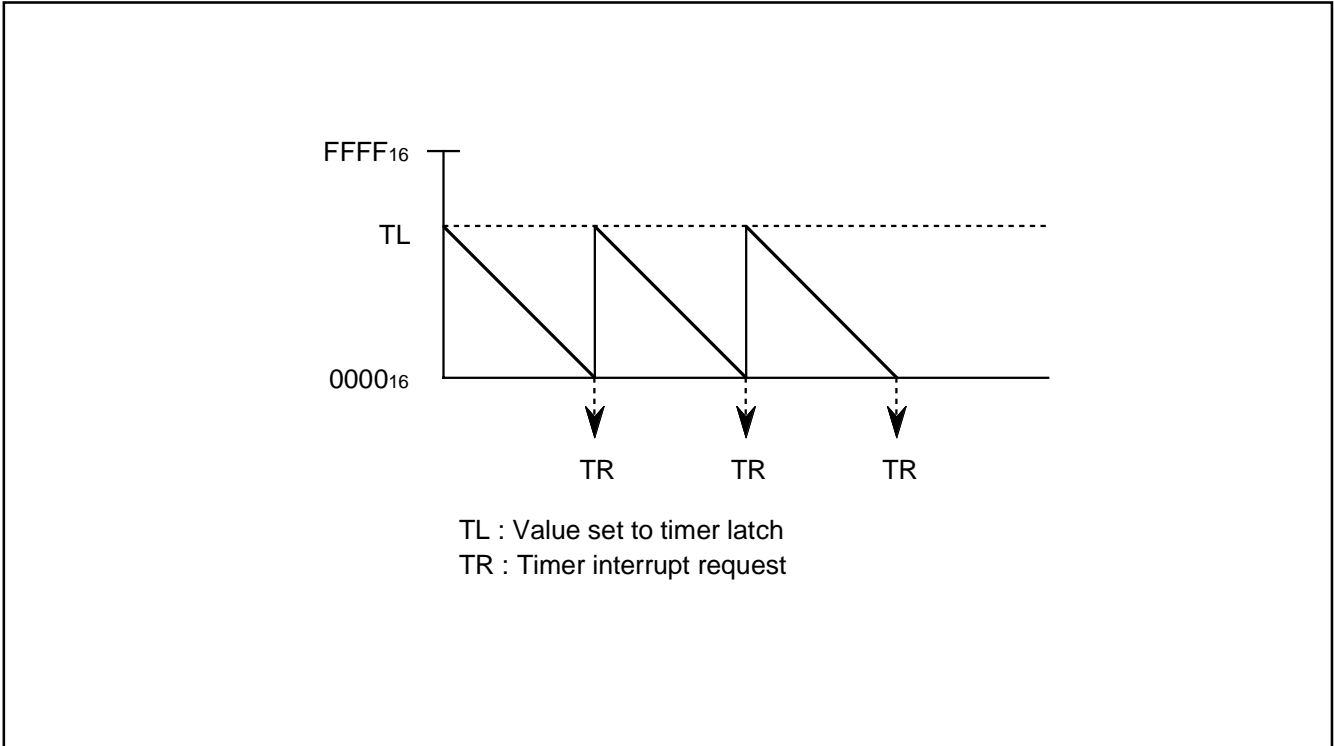
Fig. 32 Timing chart of timer/event counter mode
