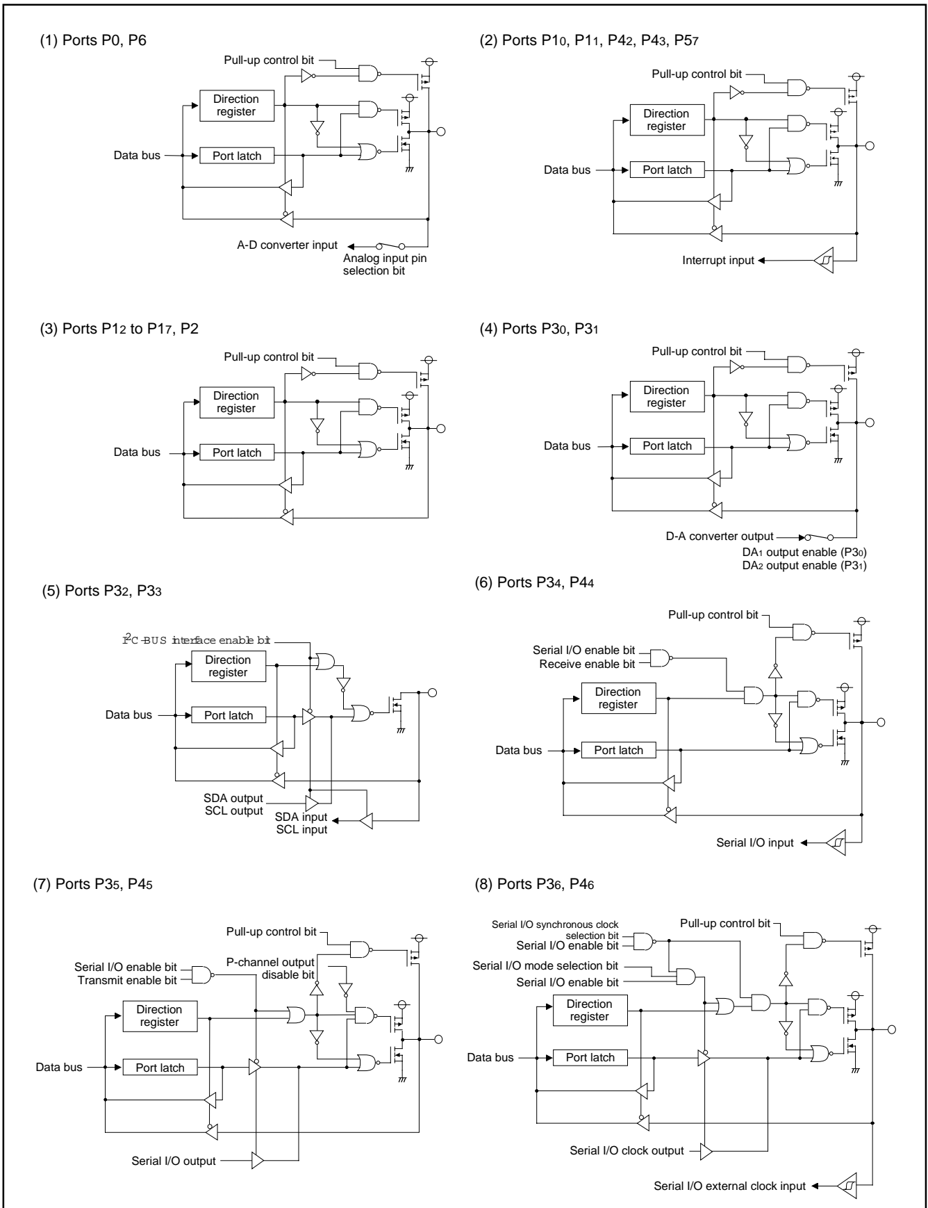
Fig. 17 Port block diagram of 3804 group (1)
