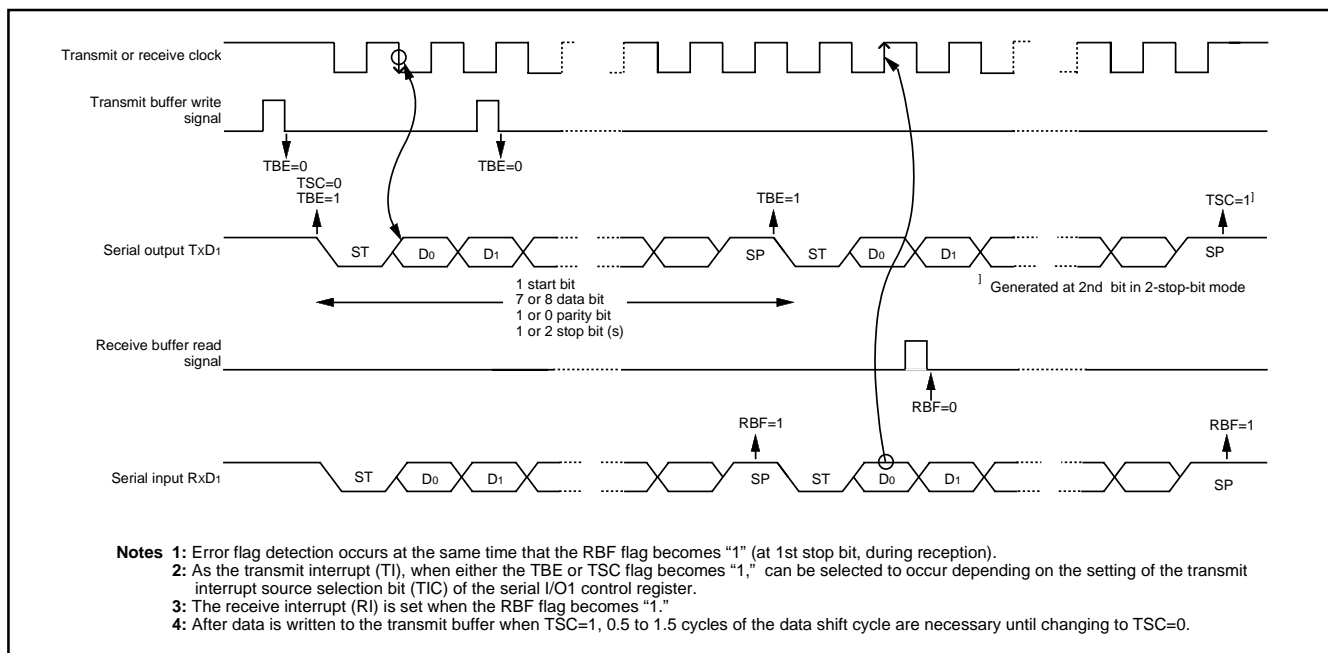
Fig. 43 Operation of UART serial I/O
