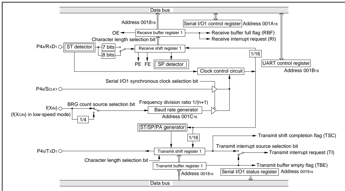
Fig. 42 Block diagram of UART serial I/O
