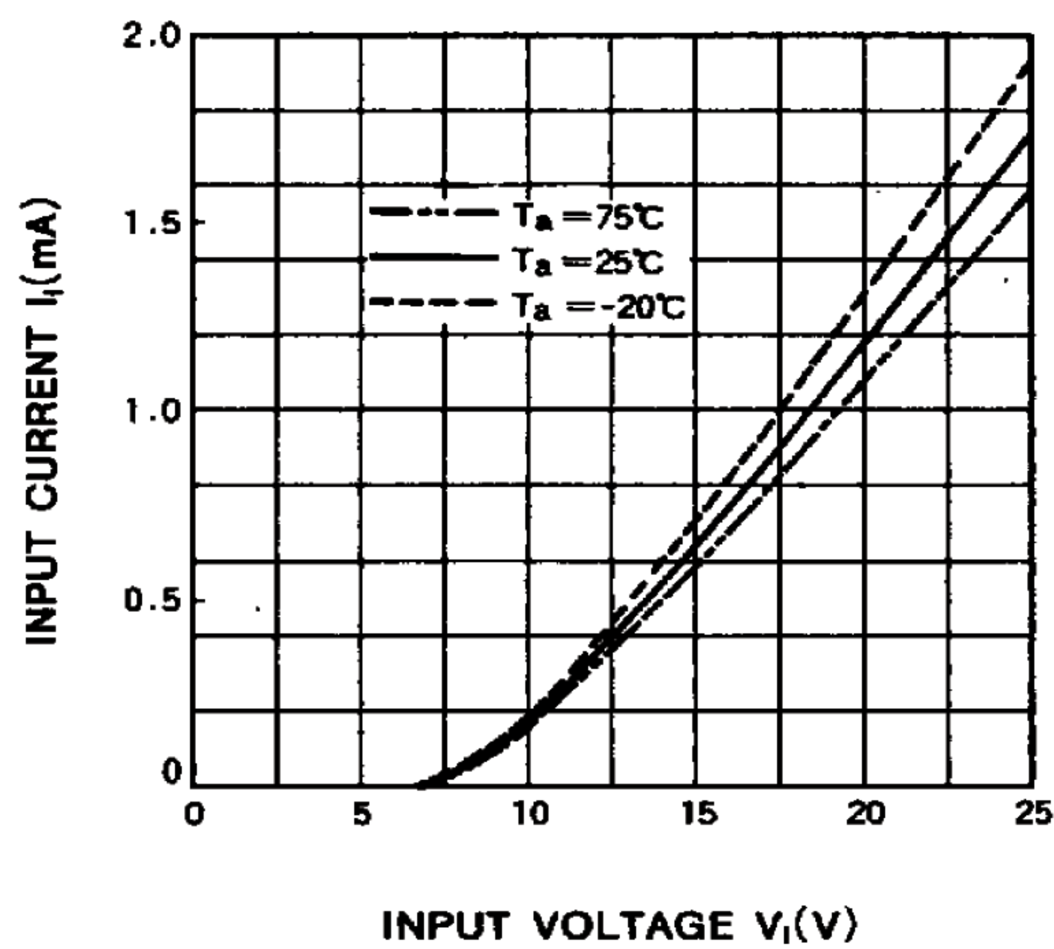
INPUT CHARACTERISTICS
