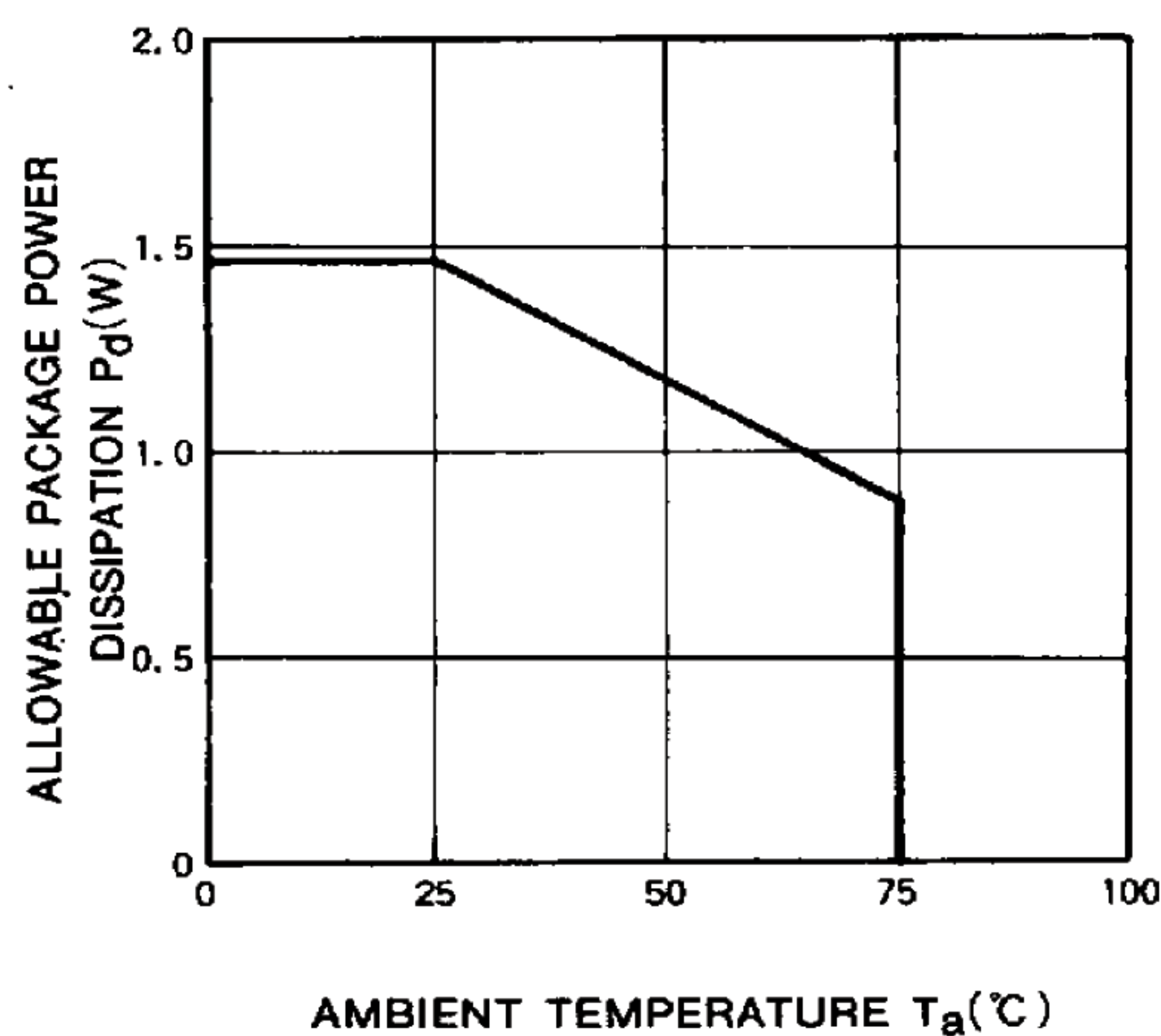
ALLOWABLE AVERAGE POWER DISSIPATION
