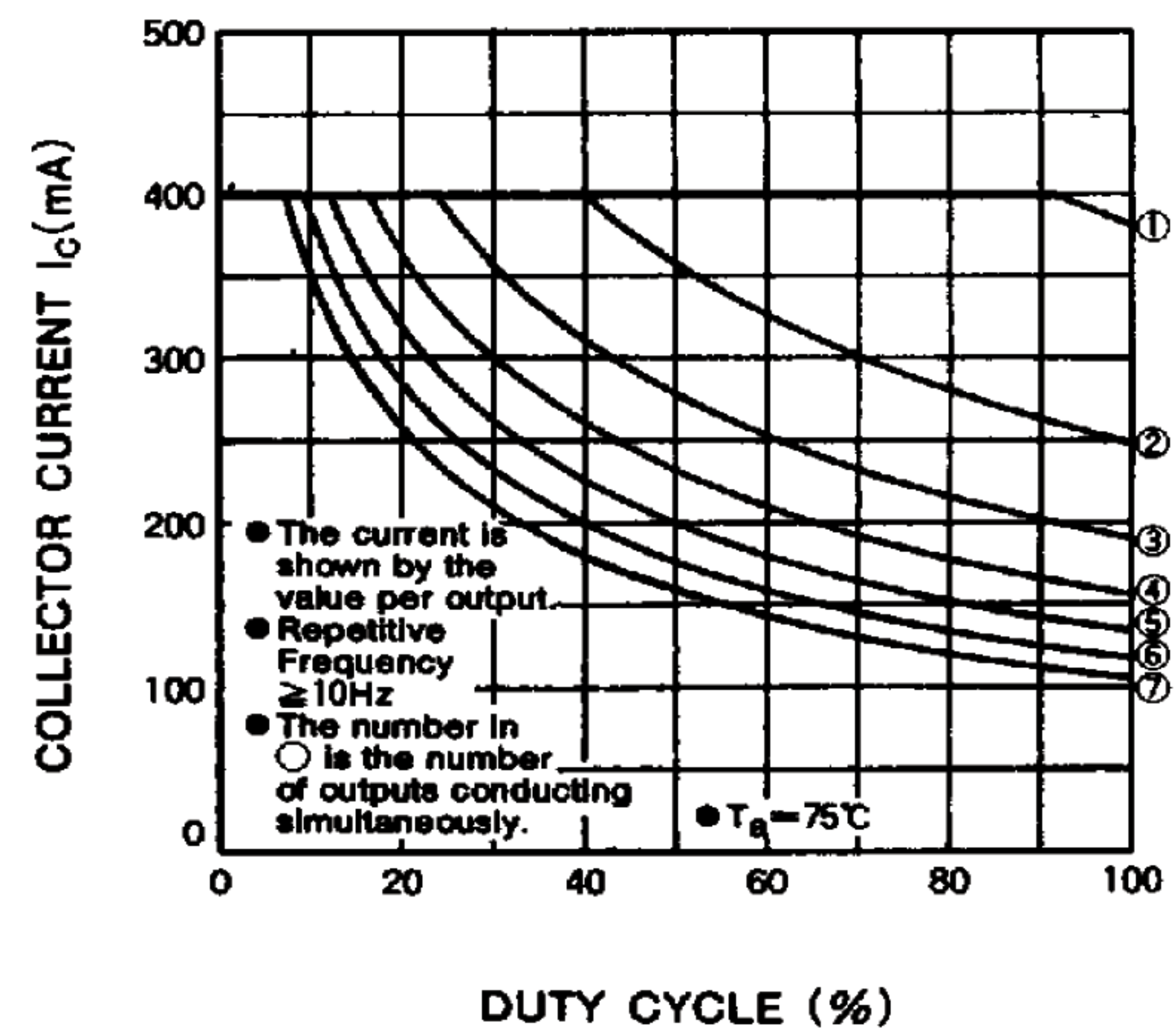
ALLOWABLE COLLECTOR CURRENT AS A FUNCTION OF DUTY CYCLE
