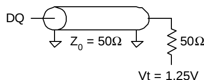
Fig. 3 OUTPUT LOAD EQUIVALENT
