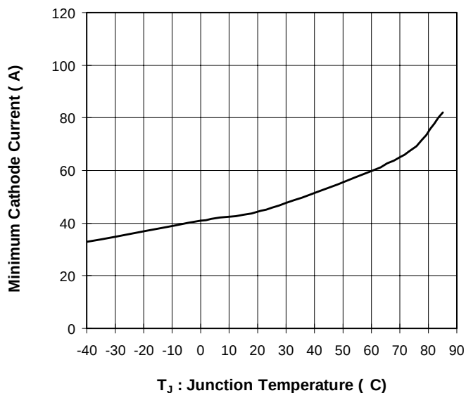
FIGURE 6 — Minimum Cathode Current for Regulation vs. Junction Temperature
