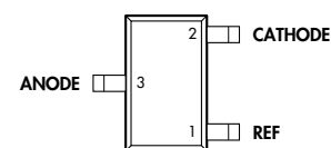
SC PACKAGE — 3-Pin (Top View)
