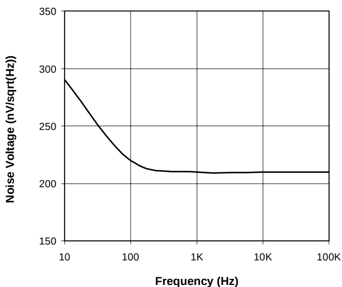
FIGURE 8 — Equivalent Input Noise Voltage vs. Frequency
