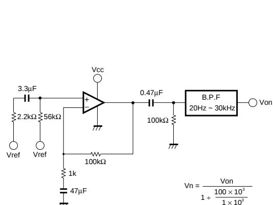
Fig. 8 Input conversion noise voltage
