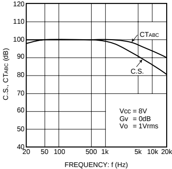
Fig. 15 Channel separation and crosstalk vs. frequency
