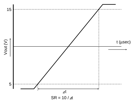
Fig. 6 Slew rate (II)
