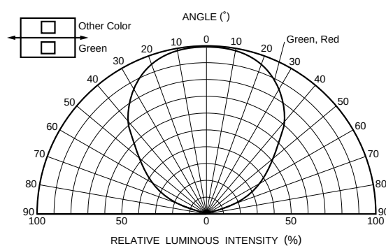
Fig. 2 Directional pattern (2)
