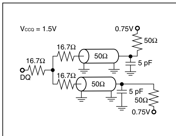
Figure 1 ( V_{CCQ} = 1.5V )
