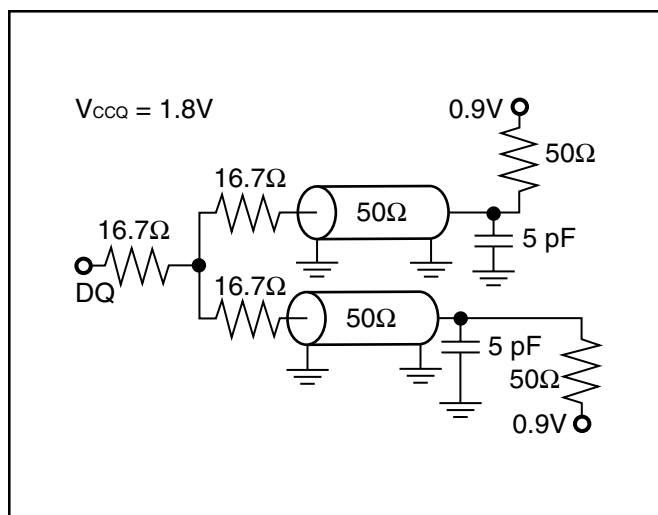
Figure 2 ( V_{CCQ} = 1.8V )
