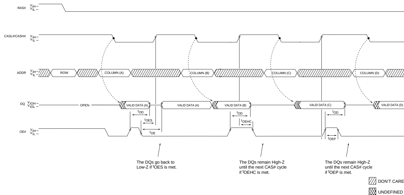
Figure 3 OUTPUT ENABLE AND DISABLE
