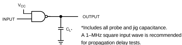
Figure 5. Test Circuit
