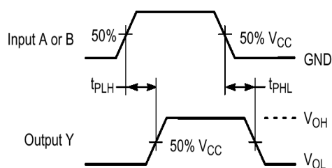
Figure 4. Switching Waveforms
