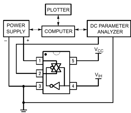
Figure 4. On Resistance Test Set-Up
