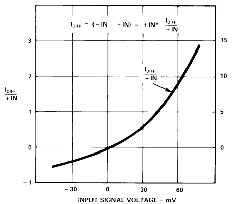
Figure 2. Differential Input Current vs. Input Signal Voltage Normalized to +IN
