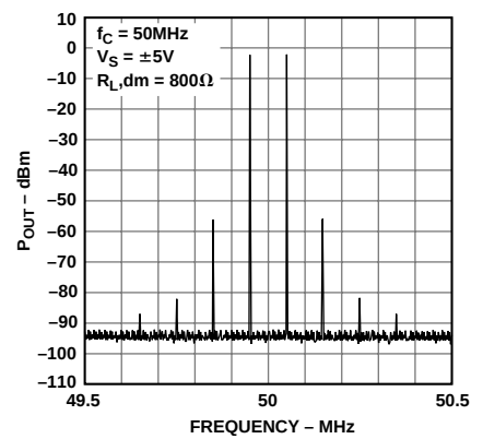
Figure 16. Intermodulation Distortion
