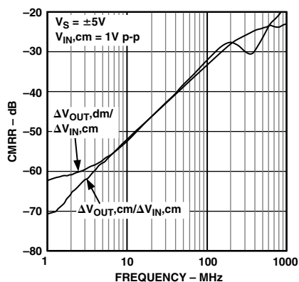
Figure 27. CMRR vs. Frequency
