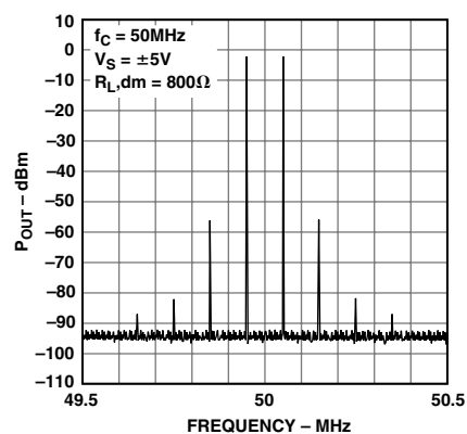
Figure 16. Intermodulation Distortion
