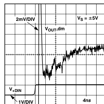
Figure 22. 0.1% Settling Time
