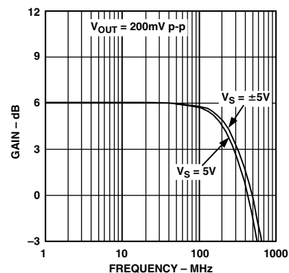
Figure 4. Small Signal Frequency Response
