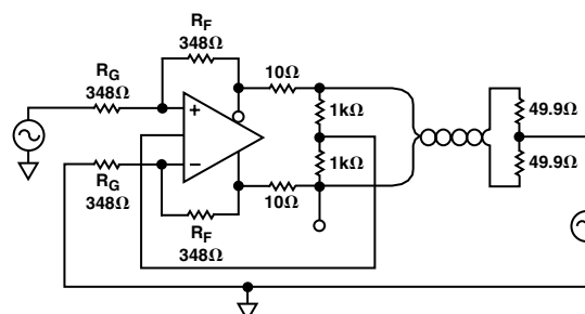
Figure 16. High Common-Mode Output Impedance Differential Amplifier
