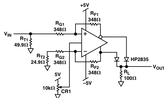
Figure 19. Full-Wave Rectifier
