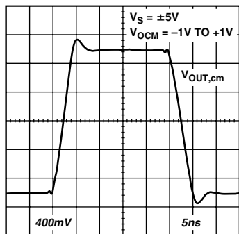
TPC 53. V_{OCM} Transient Response
