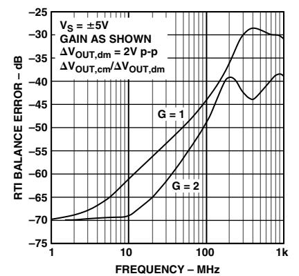
TPC 18. RTI Output Balance Error vs. Frequency
