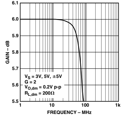
TPC 12. 0.1 dB Flatness vs. Frequency
