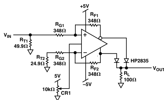
Figure 19. Full-Wave Rectifier
