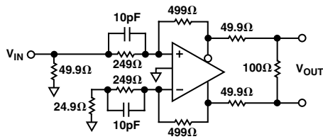
Figure 12. Frequency Boost Circuit
