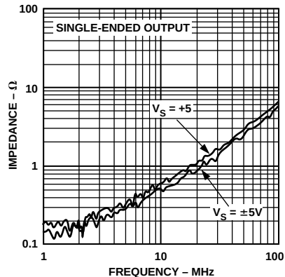
Figure 30. Output Impedance vs. Frequency
