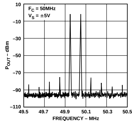
Figure 16. Intermodulation Distortion
