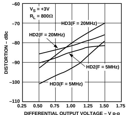
Figure 13. Harmonic Distortion vs. Differential Output Voltage
