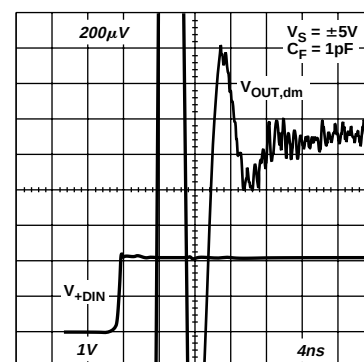
Figure 22. Settling Time
