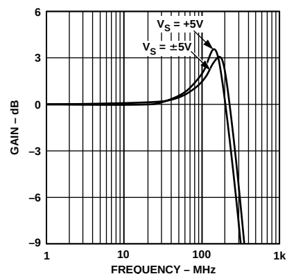
Figure 34. V_{OCM} Frequency Response
