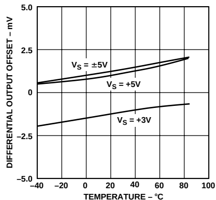
Figure 31. Output Referred Differential Offset Voltage vs. Temperature
