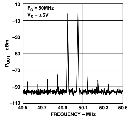
TPC 15. Intermodulation Distortion
