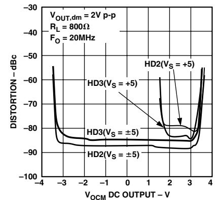
TPC 9. Harmonic Distortion vs. V_{OCM}
