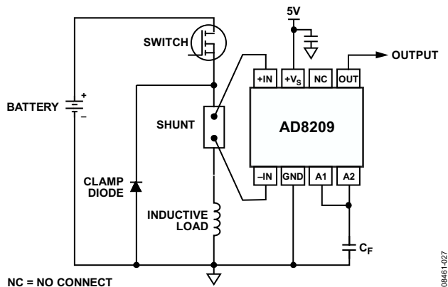
Figure 25. High-Side Switch
