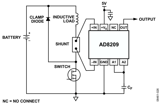
Figure 24. Low-Side Switch
