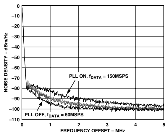
Figure 8. Phase Noise of PLL Clock Multiplier at f_{\text{OUT}} = f_{\text{DATA}}/4 at Different f_{\text{DATA}} Settings with DIV0/DIV1 Optimized, Using R&S FSEA30 Spectrum Analyzer
