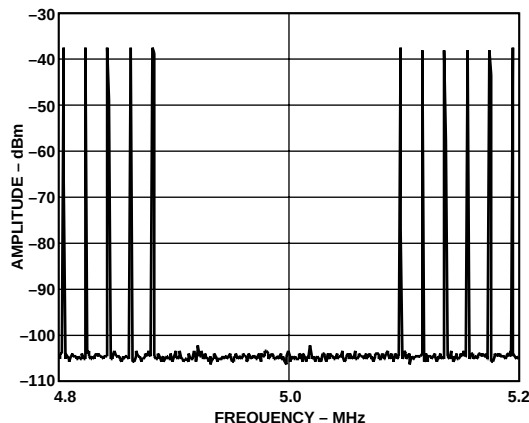
Figure 35b. Notch in missing bin at 5 MHz is down >60 dB. Peak amplitude = 0 dBm.
