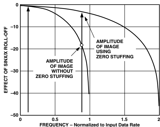
Figure 33. Effects of Pseudo Zero Stuffing on Spectrum of AD9755
