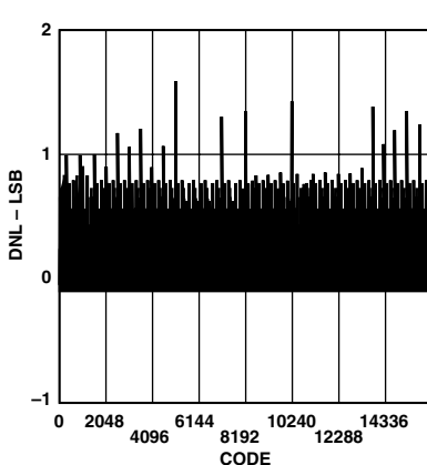
TPC 17. Typical DNL
