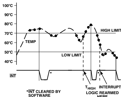
Figure 7. Operation of \overline{\text{INT}} Output
