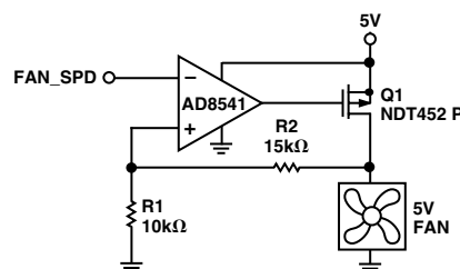
Figure 5a. 5 V Fan Circuit with Op Amp
