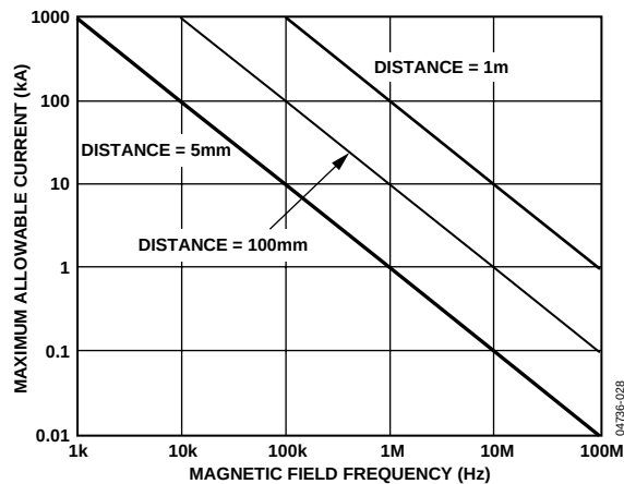
Figure 28. Maximum Allowable Current for Various Current-to-ADM2483 Spacings
