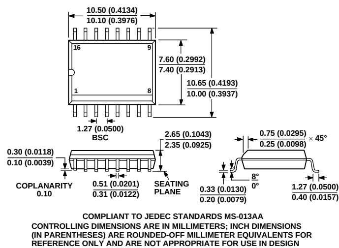
Figure 31. 16-Lead Standard Small Outline Package [SOIC] Wide Body (RW-16) Dimensions shown in millimeters and (inches)
