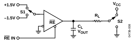
Figure 8. Receiver Enable/Disable
