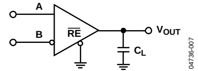
Figure 7. Receiver Propagation Delay
