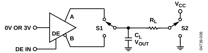
Figure 6. Driver Enable/Disable
