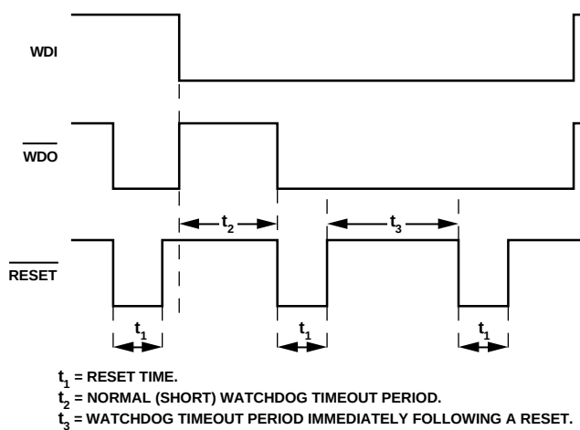
Figure 3. Watchdog Timeout Period and Reset Active Time
