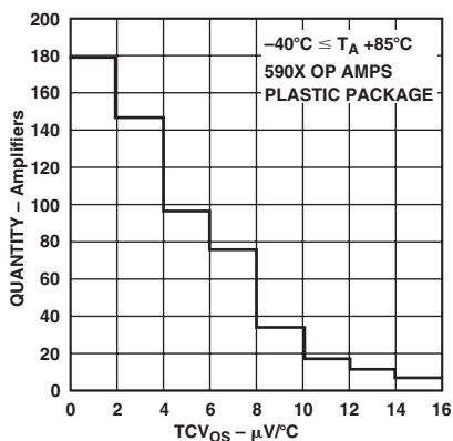
TPC 8. OP283 Input Offset Voltage Drift ( TCV_{OS} ) Distribution @ \pm 15 V
