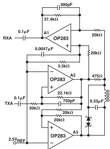
Figure 2. Direct Access Arrangement
