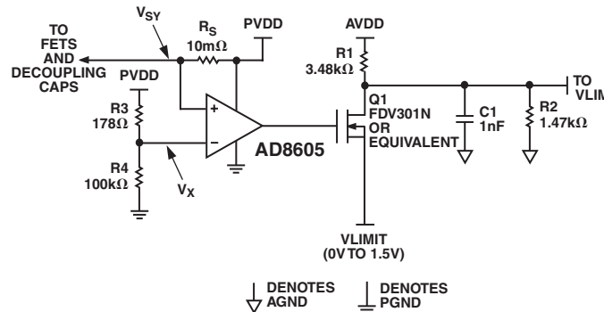
Figure 21. Setting a Maximum Output Current Limit
