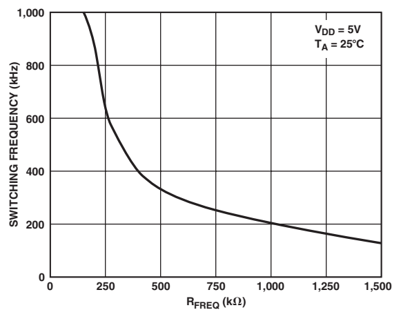
TPC 6. Switching Frequency vs. R_{FREQ}
