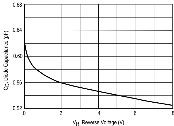
Figure 4. Capacitance
