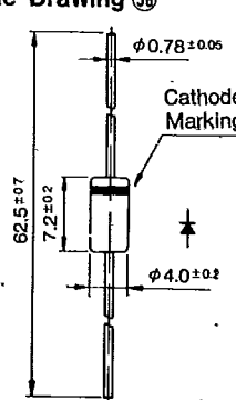
Outline Drawing ⑤8
