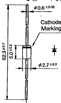
Outline Drawing ⑤6
