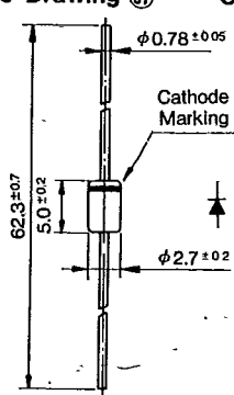
Outline Drawing ⑥1
