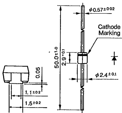
Outline Drawing ⑥0
