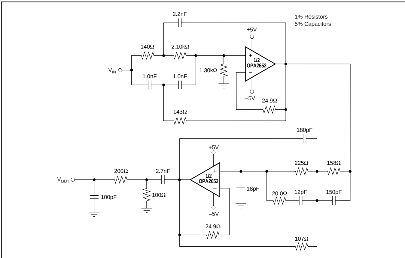
FIGURE 3. Bandpass Filter.
