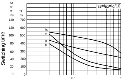
Switching Speeds
