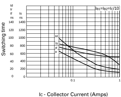
Switching Speeds
