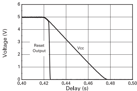
Reset Low Switching Characteristic - ZXCM209L
