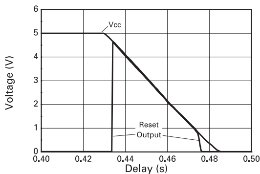
Reset Low Switching Characteristic - ZXCM210L
